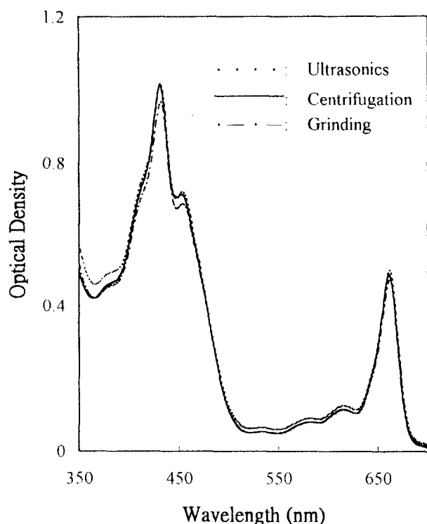
Fig. 1. Ultraviolet-visible spectra of chlorophyll of moso bamboo ( Phyllostachys pubescens ) culm obtained using different extraction methods
