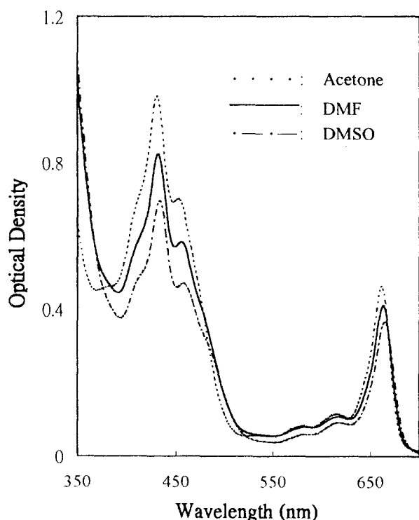
Fig. 2. Ultraviolet-visible spectra of chlorophyll of moso bamboo ( Phyllostachys pubescens ) culm extracted by ultrasonics in acetone, N,N -dimethylformamide (DMF), and dimethylsulfoxide (DMSO)
