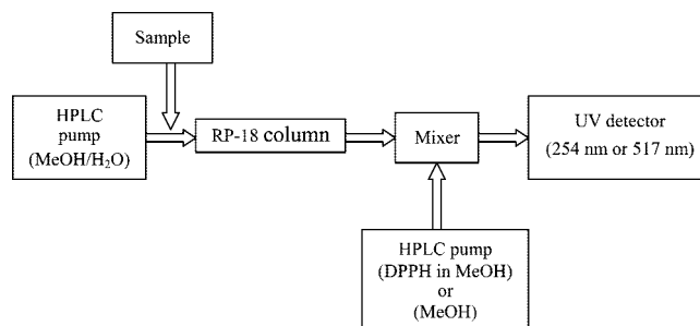
Figure 2. Instrumental setup for the HPLC-DPPH online detection of radical-scavenging compounds.
