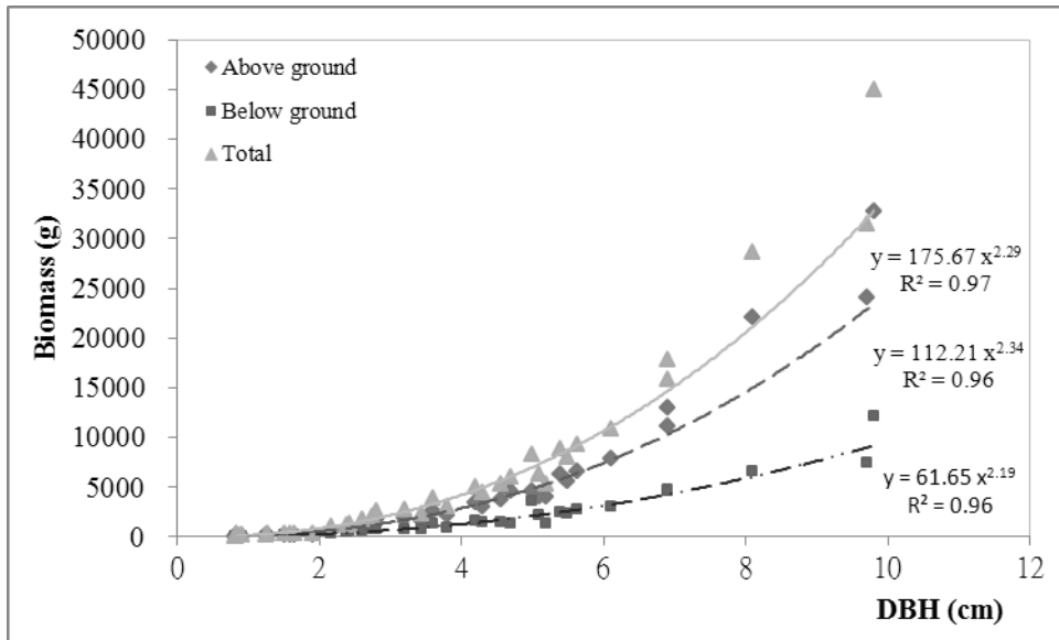
Fig. 2 Relationship between biomass and the diameter at breast height (DBH) of mahogany saplings.
