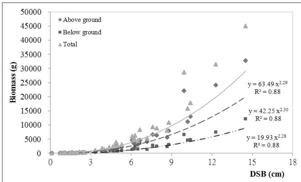
Fig. 3 Relationship between biomass and the diameter at stem base (DSB) of mahogany saplings.
