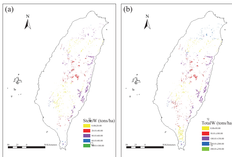
Fig. 7. Carbon stock of camphor trees ( \text{tons ha}^{-1} ). (a) stem part; (b) aboveground part.
