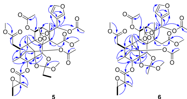
Figure 5. COSY (bold bond) and selected HMBC (arrow) correlations of 5 and 6 .
